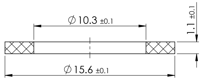
SECTION X-X
